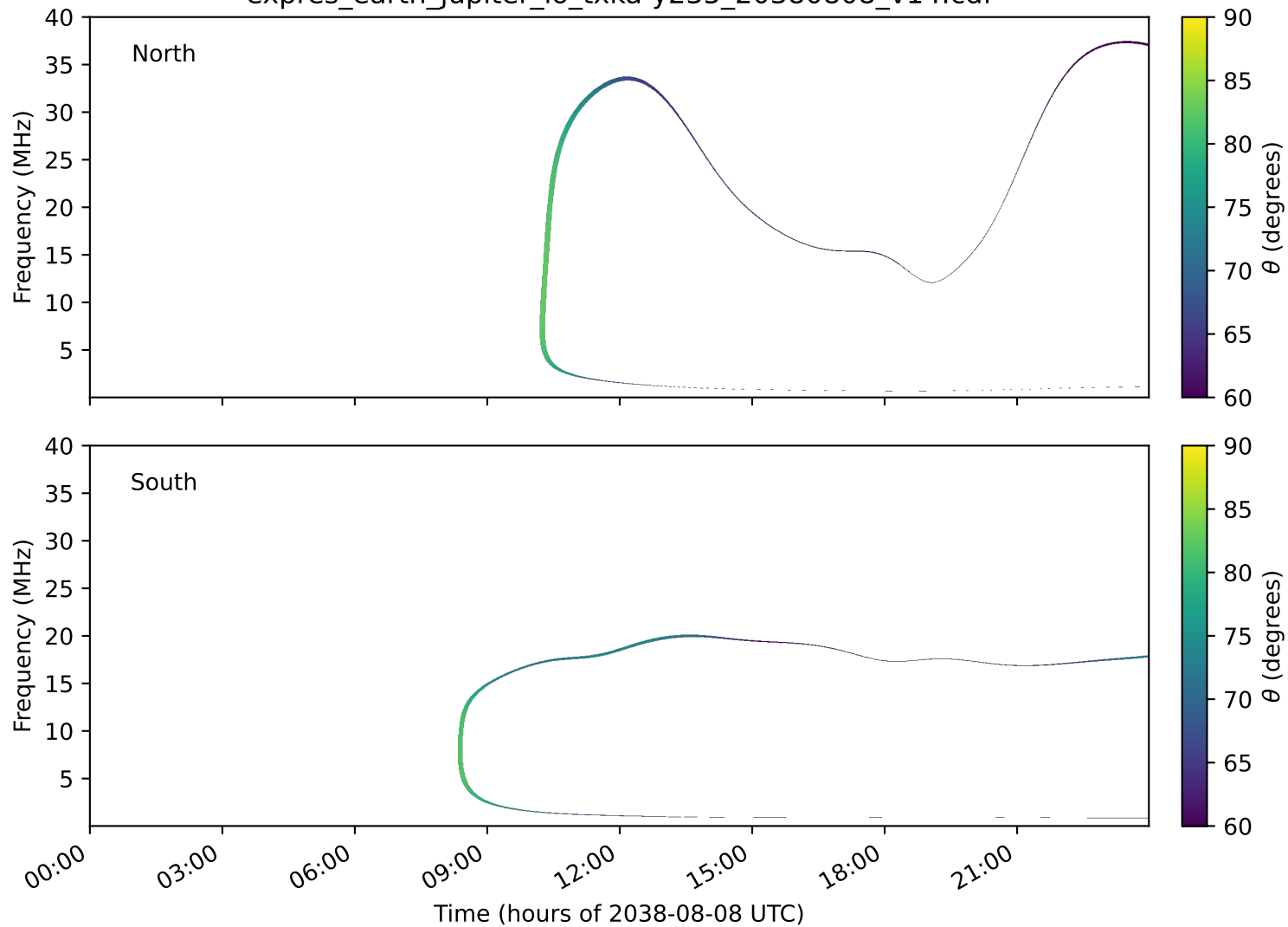
expres_earth_jupiter_io_txka-y235_20380808_v14.cdf
