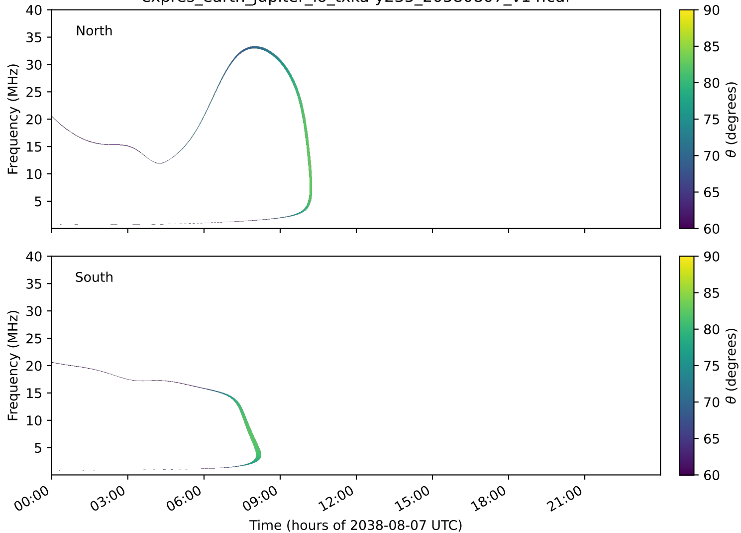
expres_earth_jupiter_io_txka-y235_20380807_v14.cdf
