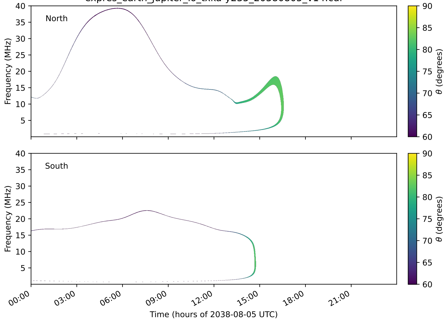
expres_earth_jupiter_io_txka-y235_20380805_v14.cdf
