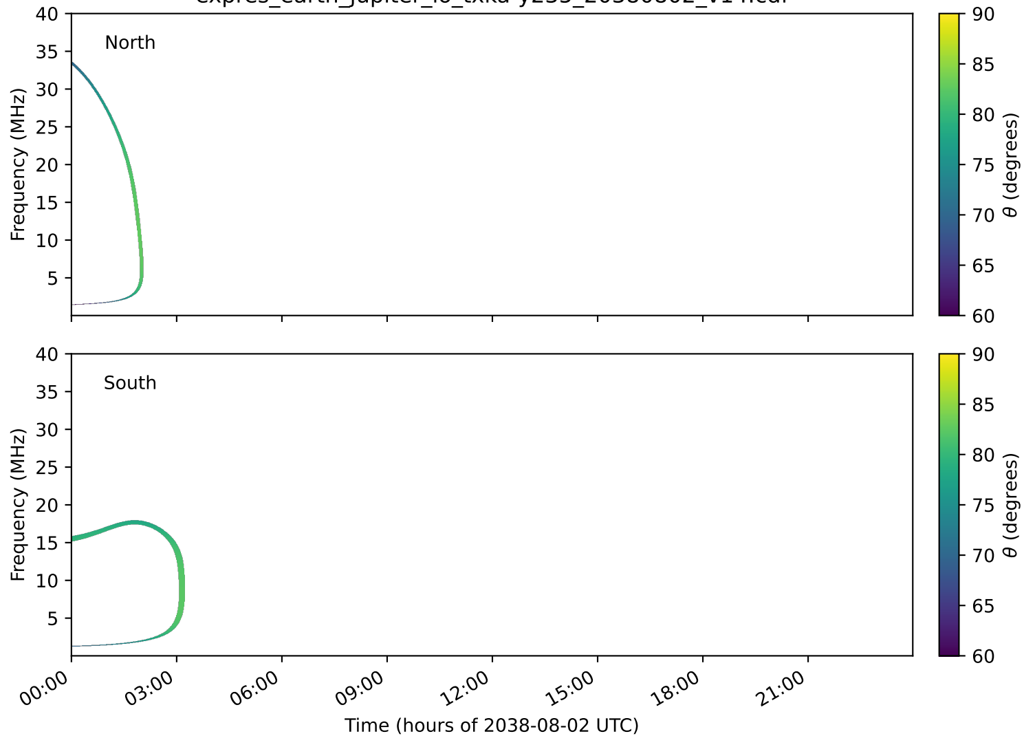
expres_earth_jupiter_io_txka-y235_20380802_v14.cdf
