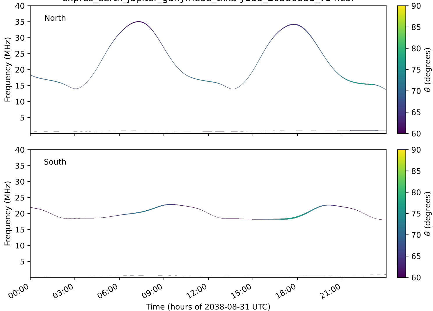
expres_earth_jupiter_ganymede_txka-y235_20380831_v14.cdf
