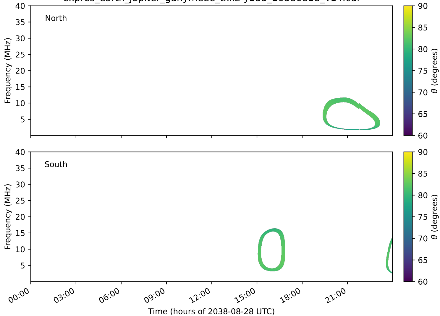
expres_earth_jupiter_ganymede_txka-y235_20380828_v14.cdf
