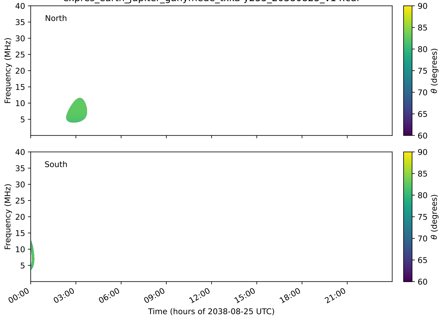
expres_earth_jupiter_ganymede_txka-y235_20380825_v14.cdf
