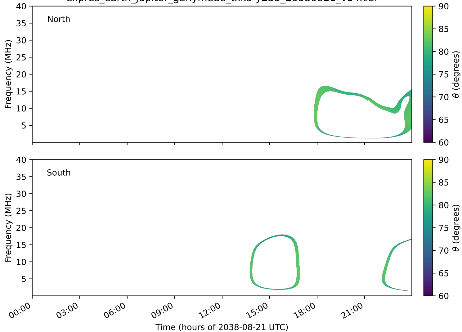
expres_earth_jupiter_ganymede_txka-y235_20380821_v14.cdf
