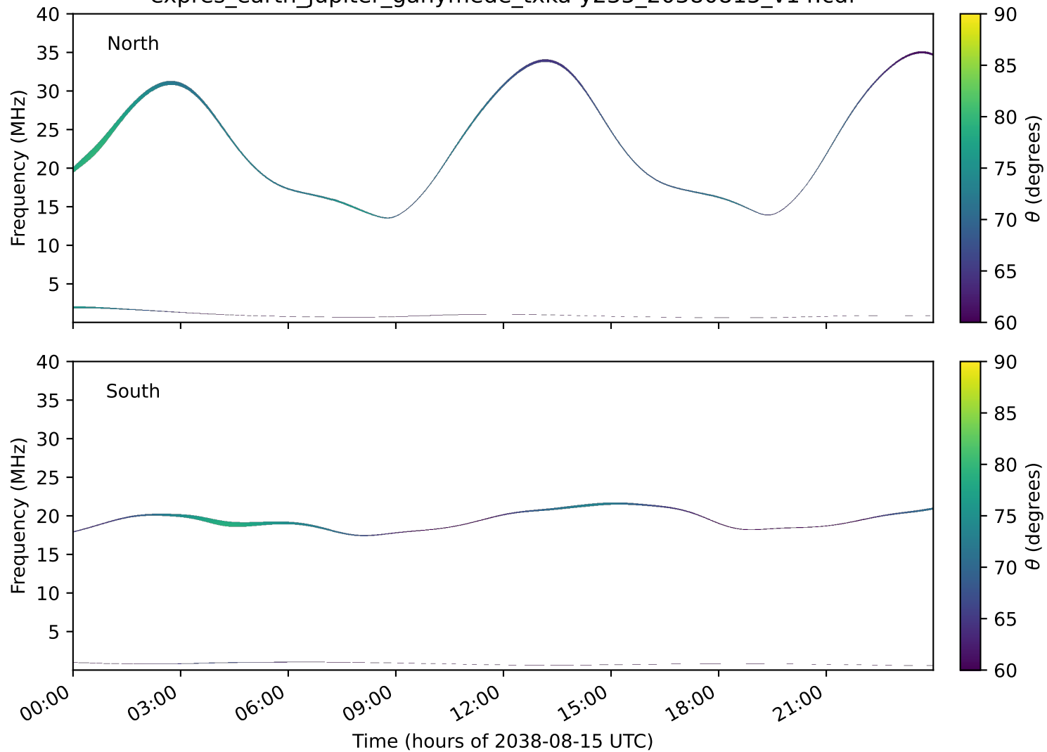
expres_earth_jupiter_ganymede_txka-y235_20380815_v14.cdf
