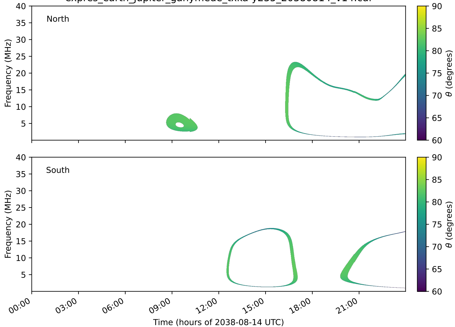
expres_earth_jupiter_ganymede_txka-y235_20380814_v14.cdf
