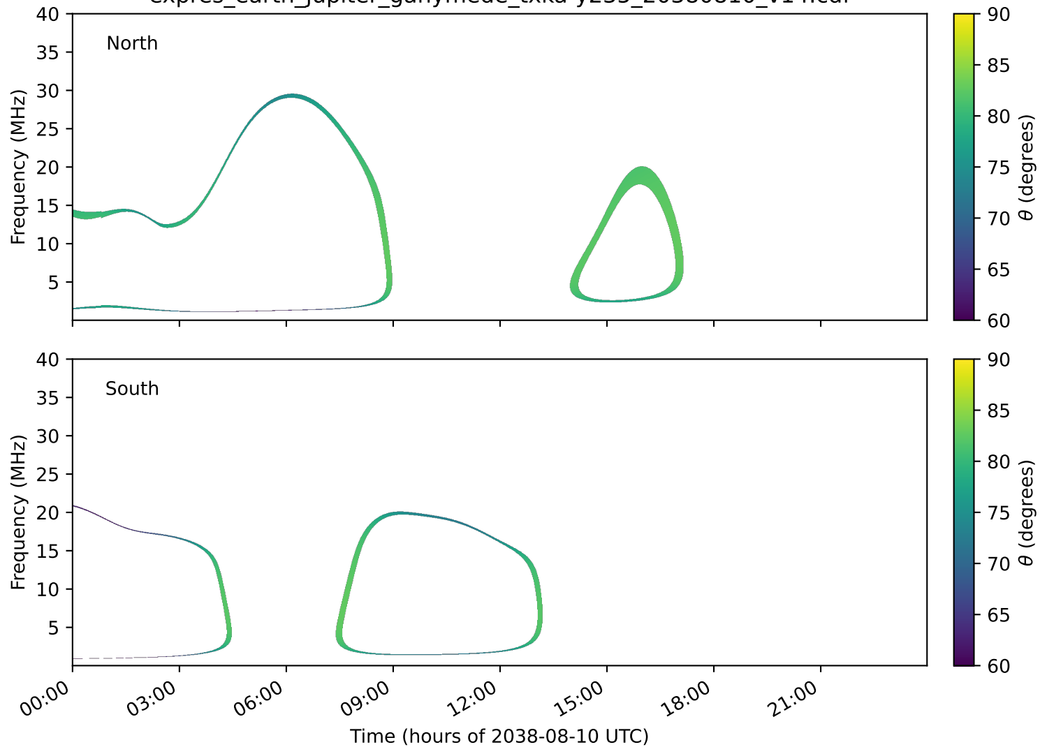
expres_earth_jupiter_ganymede_txka-y235_20380810_v14.cdf
