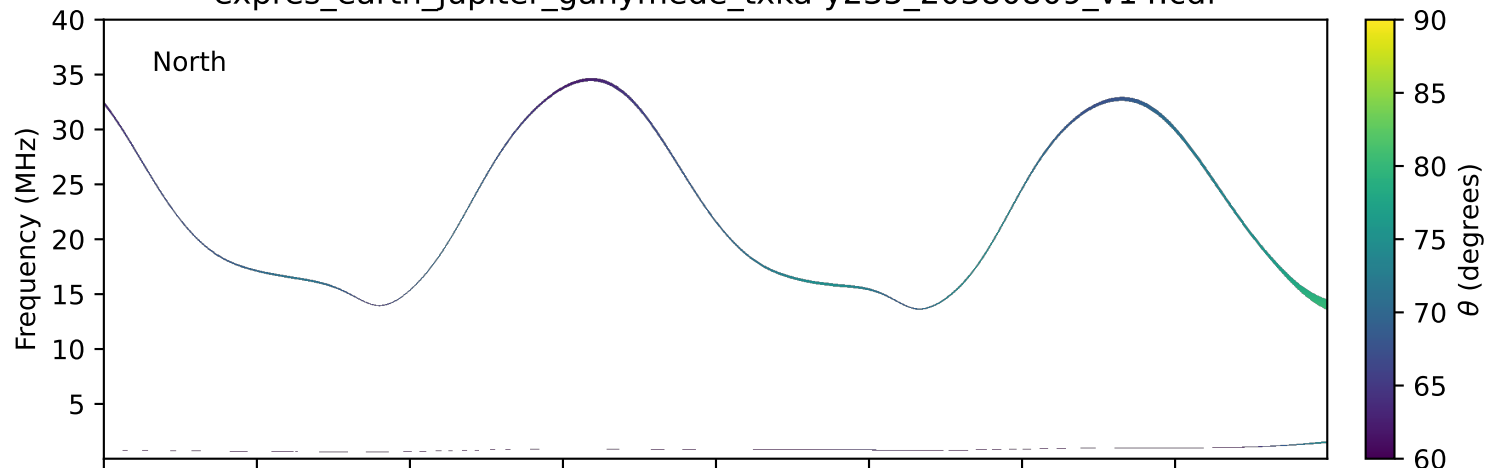
expres_earth_jupiter_ganymede_txka-y235_20380809_v14.cdf
