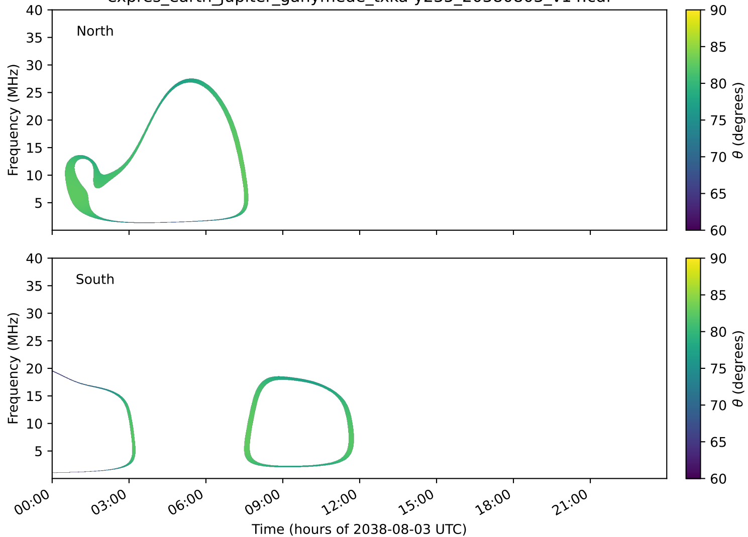
expres_earth_jupiter_ganymede_txka-y235_20380803_v14.cdf
