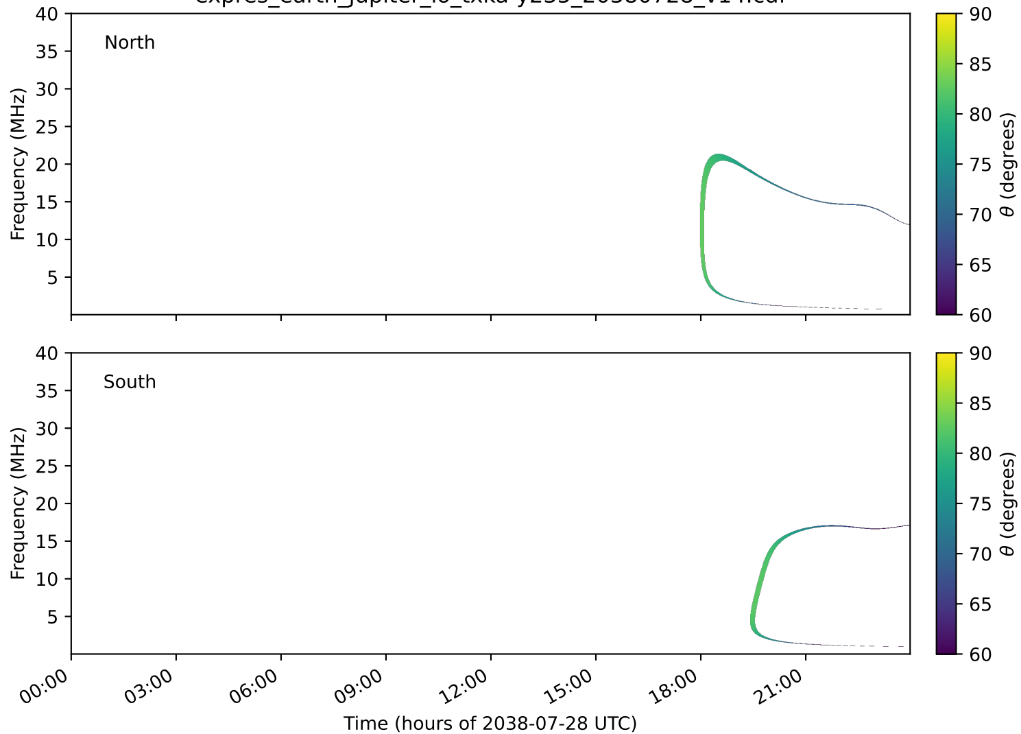
expres_earth_jupiter_io_txka-y235_20380728_v14.cdf
