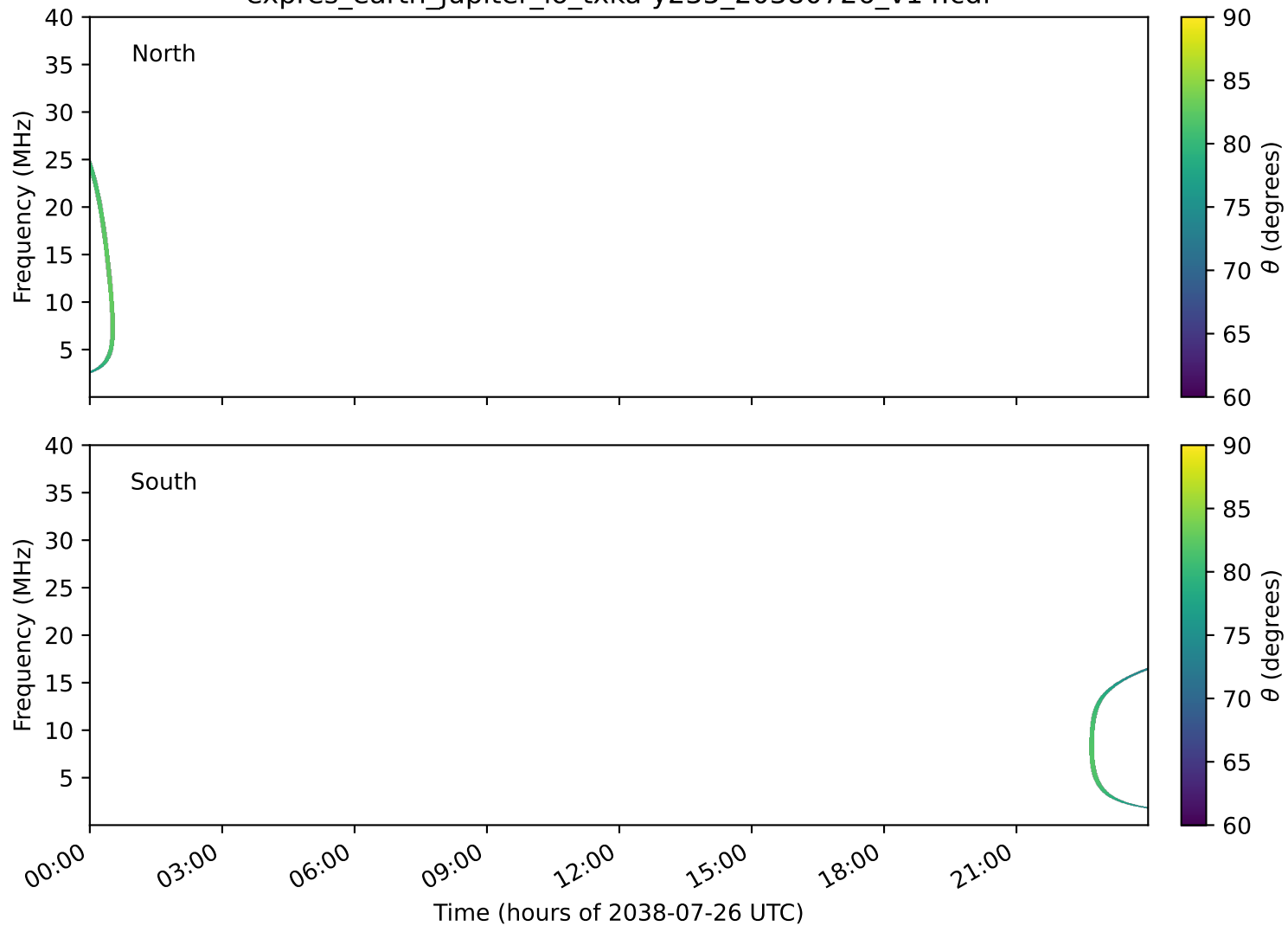
expres_earth_jupiter_io_txka-y235_20380726_v14.cdf
