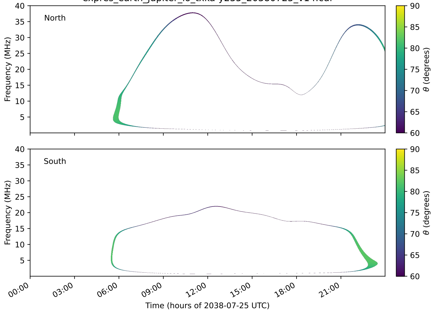
expres_earth_jupiter_io_txka-y235_20380725_v14.cdf
