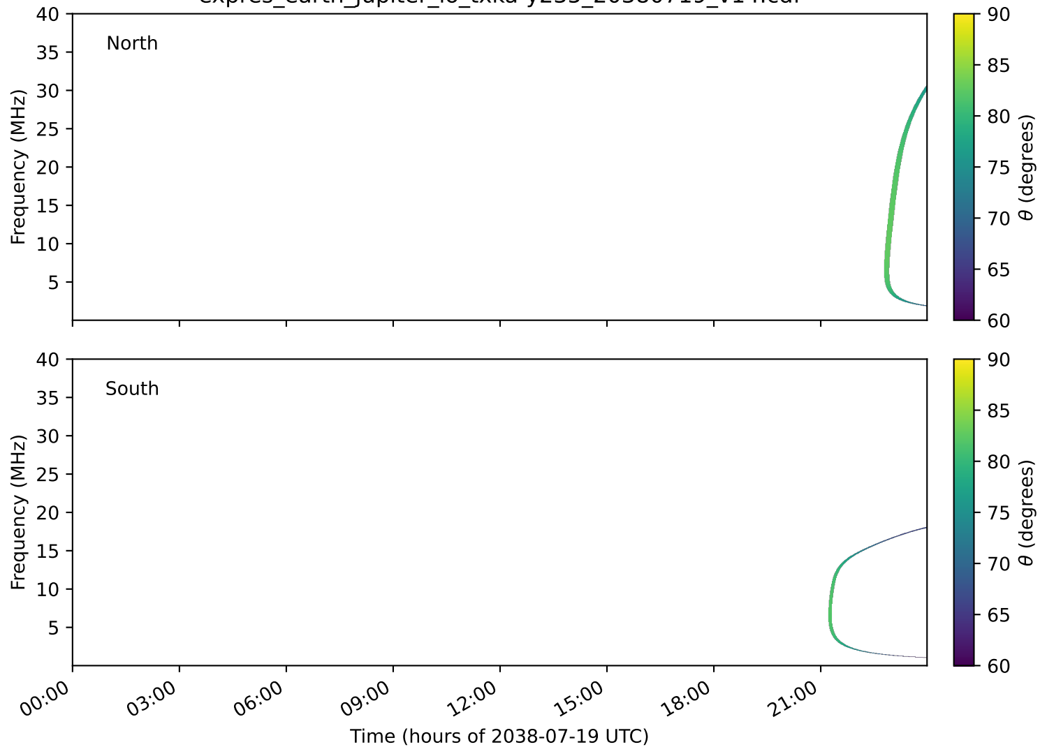
expres_earth_jupiter_io_txka-y235_20380719_v14.cdf
