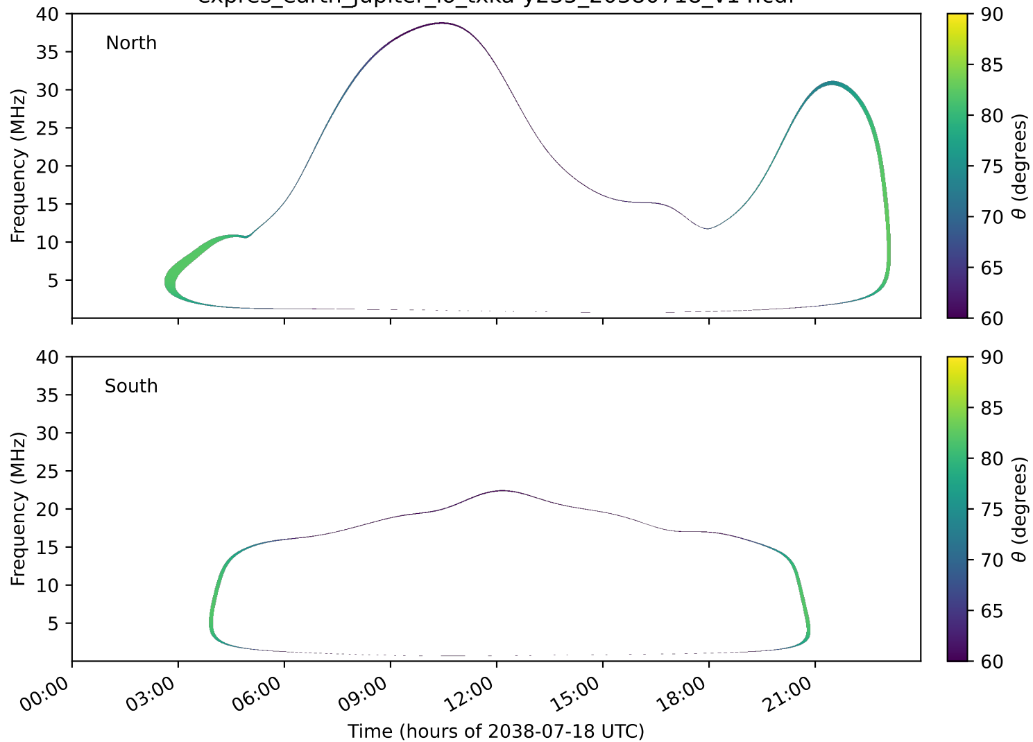
expres_earth_jupiter_io_txka-y235_20380718_v14.cdf
