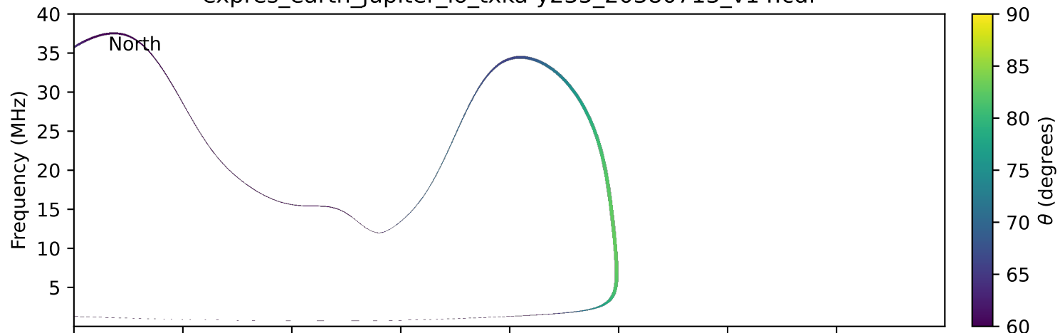
expres_earth_jupiter_io_txka-y235_20380713_v14.cdf
