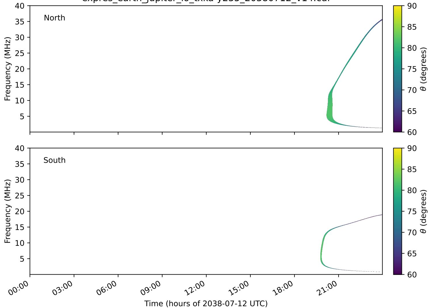
expres_earth_jupiter_io_txka-y235_20380712_v14.cdf
