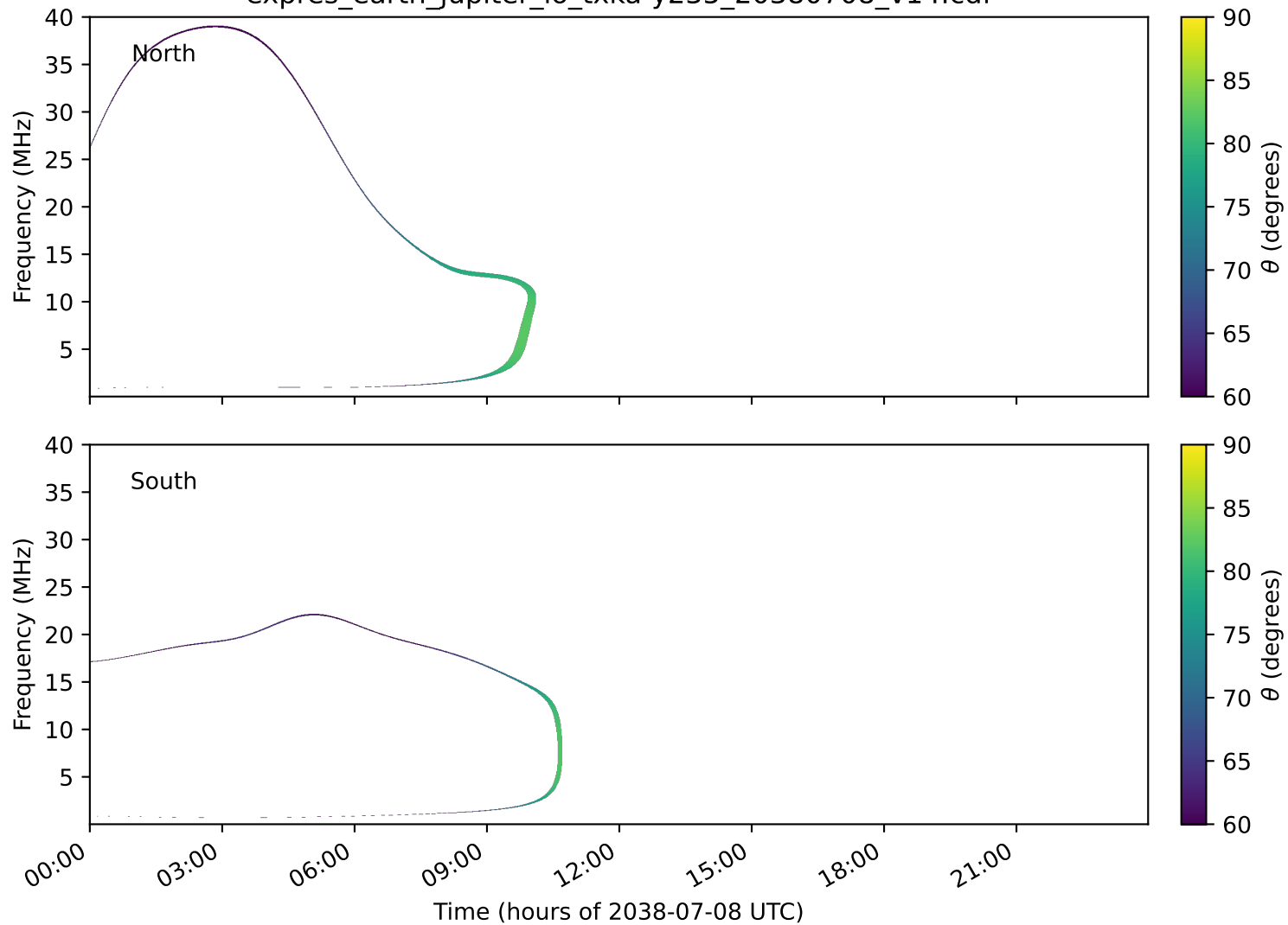
expres_earth_jupiter_io_txka-y235_20380708_v14.cdf
