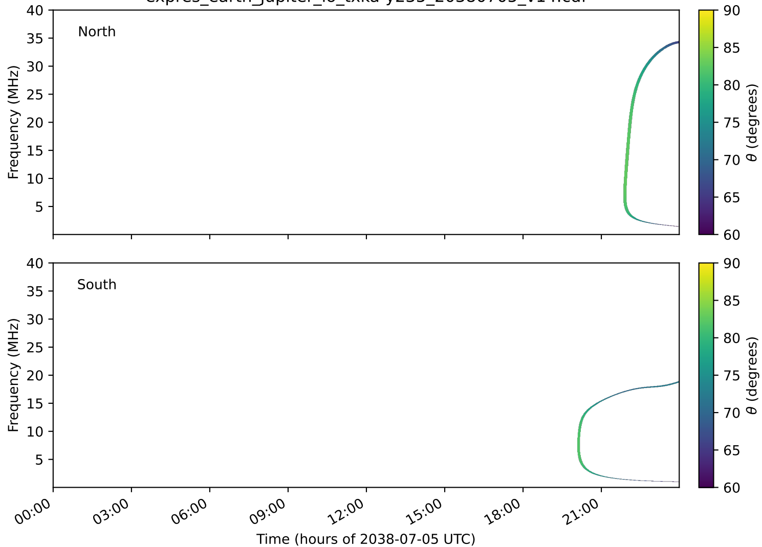
expres_earth_jupiter_io_txka-y235_20380705_v14.cdf
