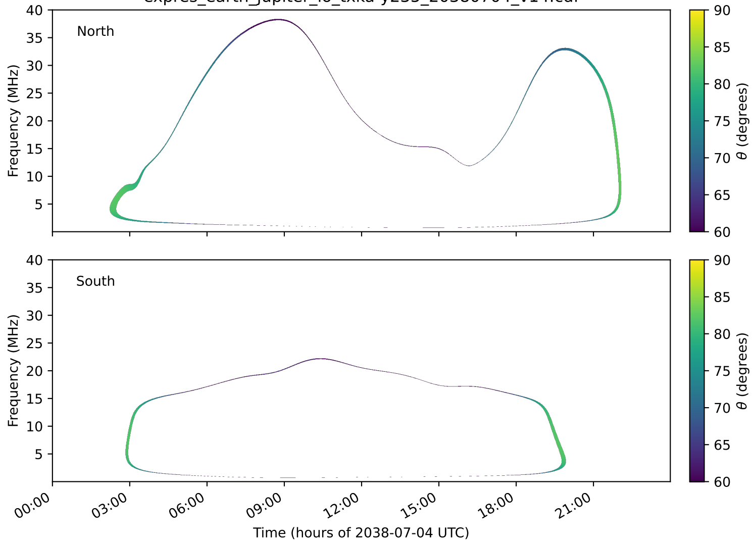
expres_earth_jupiter_io_txka-y235_20380704_v14.cdf
