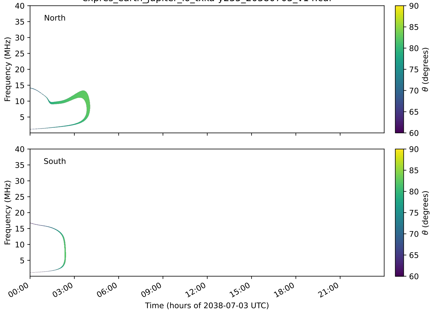
expres_earth_jupiter_io_txka-y235_20380703_v14.cdf
