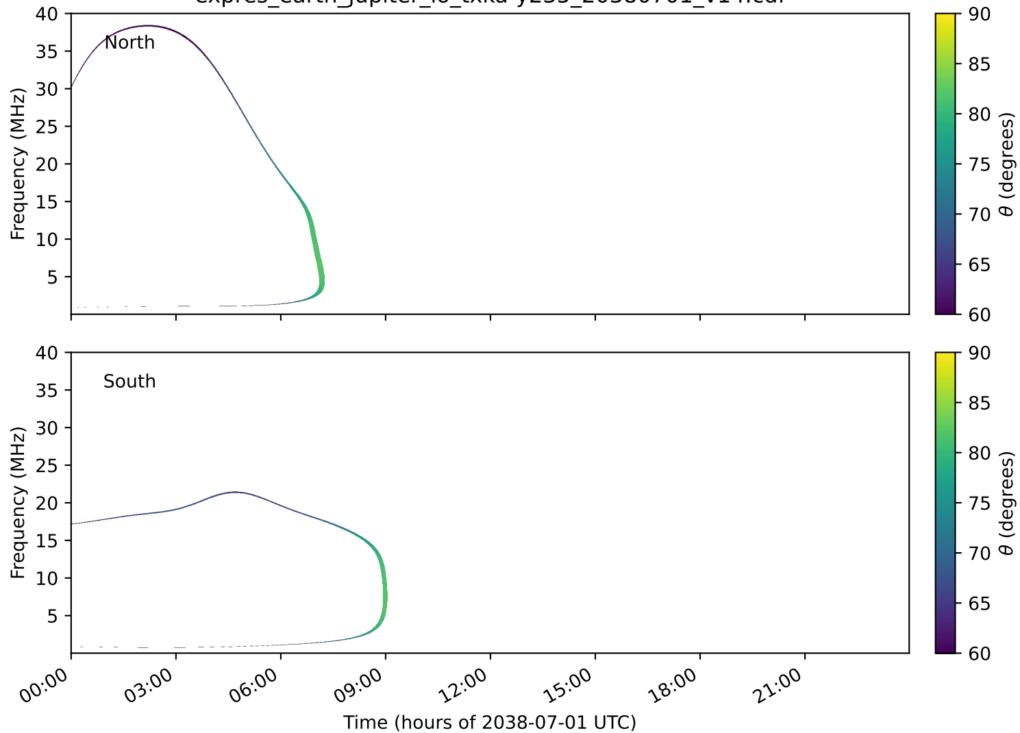
expres_earth_jupiter_io_txka-y235_20380701_v14.cdf
