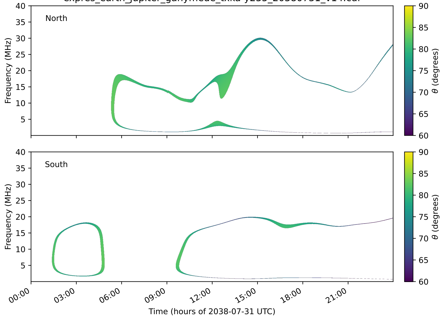
expres_earth_jupiter_ganymede_txka-y235_20380731_v14.cdf
