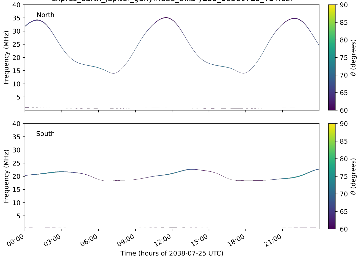
expres_earth_jupiter_ganymede_txka-y235_20380725_v14.cdf
