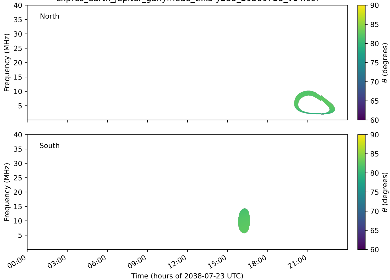
expres_earth_jupiter_ganymede_txka-y235_20380723_v14.cdf
