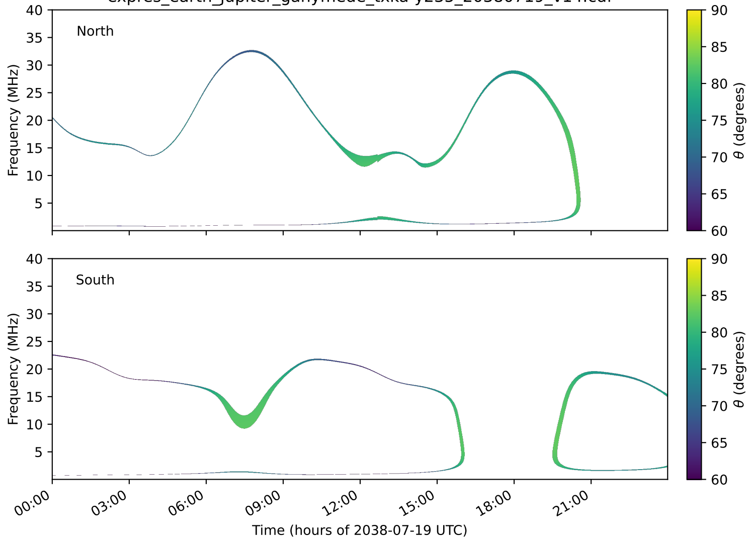
expres_earth_jupiter_ganymede_txka-y235_20380719_v14.cdf
