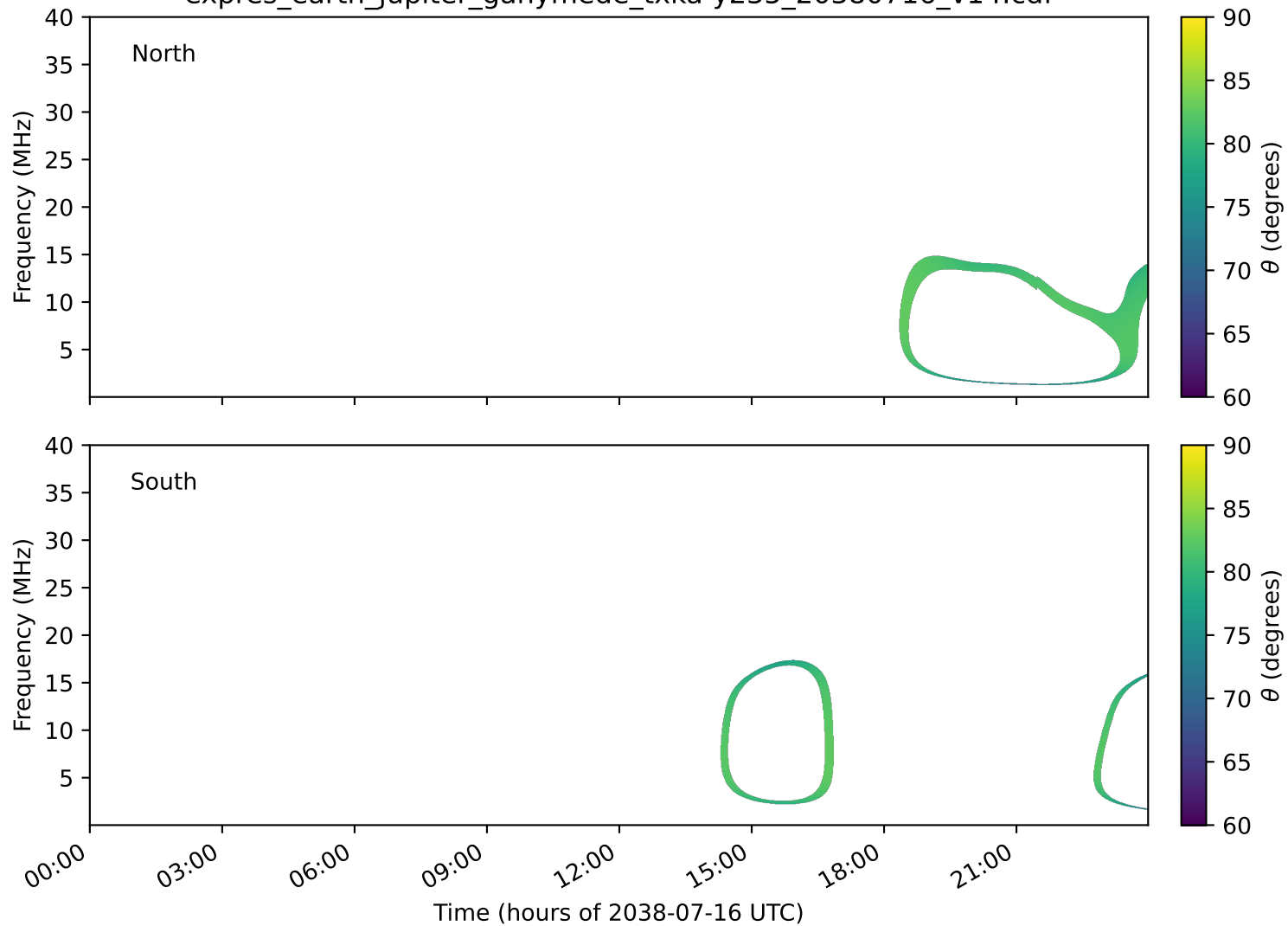
expres_earth_jupiter_ganymede_txka-y235_20380716_v14.cdf
