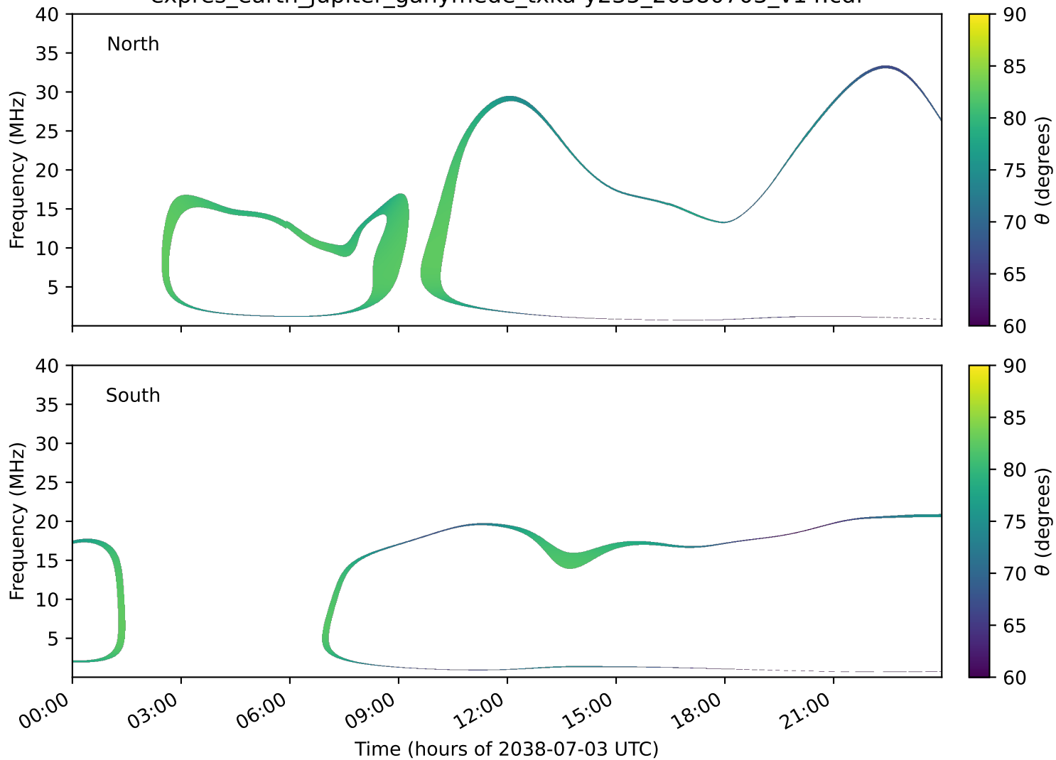
expres_earth_jupiter_ganymede_txka-y235_20380703_v14.cdf
