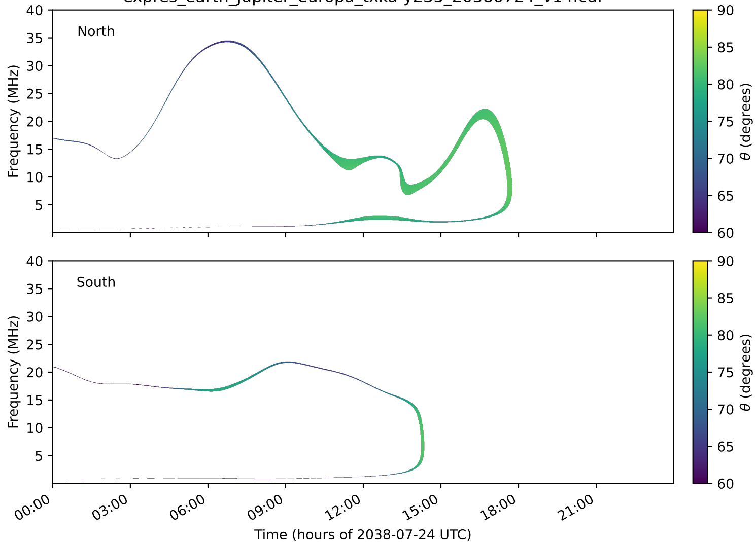
expres_earth_jupiter_europa_txka-y235_20380724_v14.cdf
