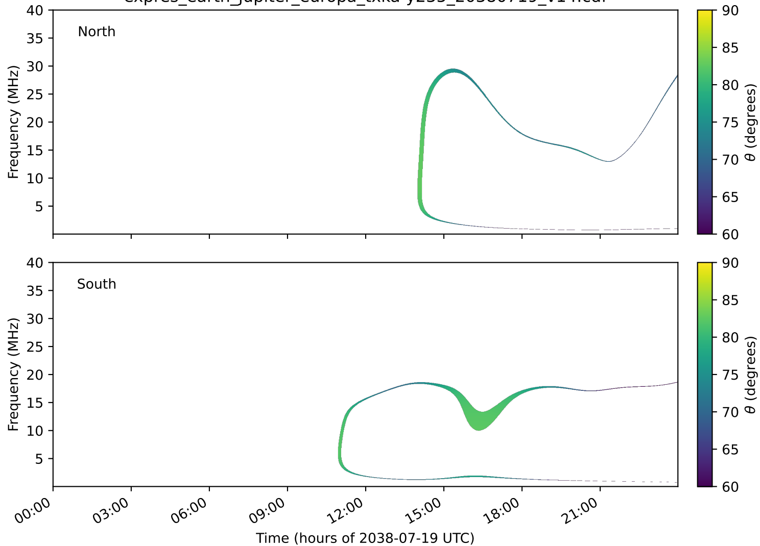
expres_earth_jupiter_europa_txka-y235_20380719_v14.cdf
