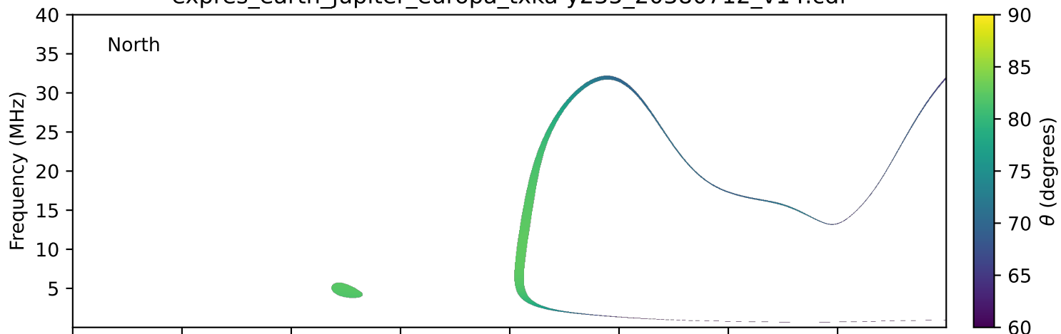
expres_earth_jupiter_europa_txka-y235_20380712_v14.cdf
