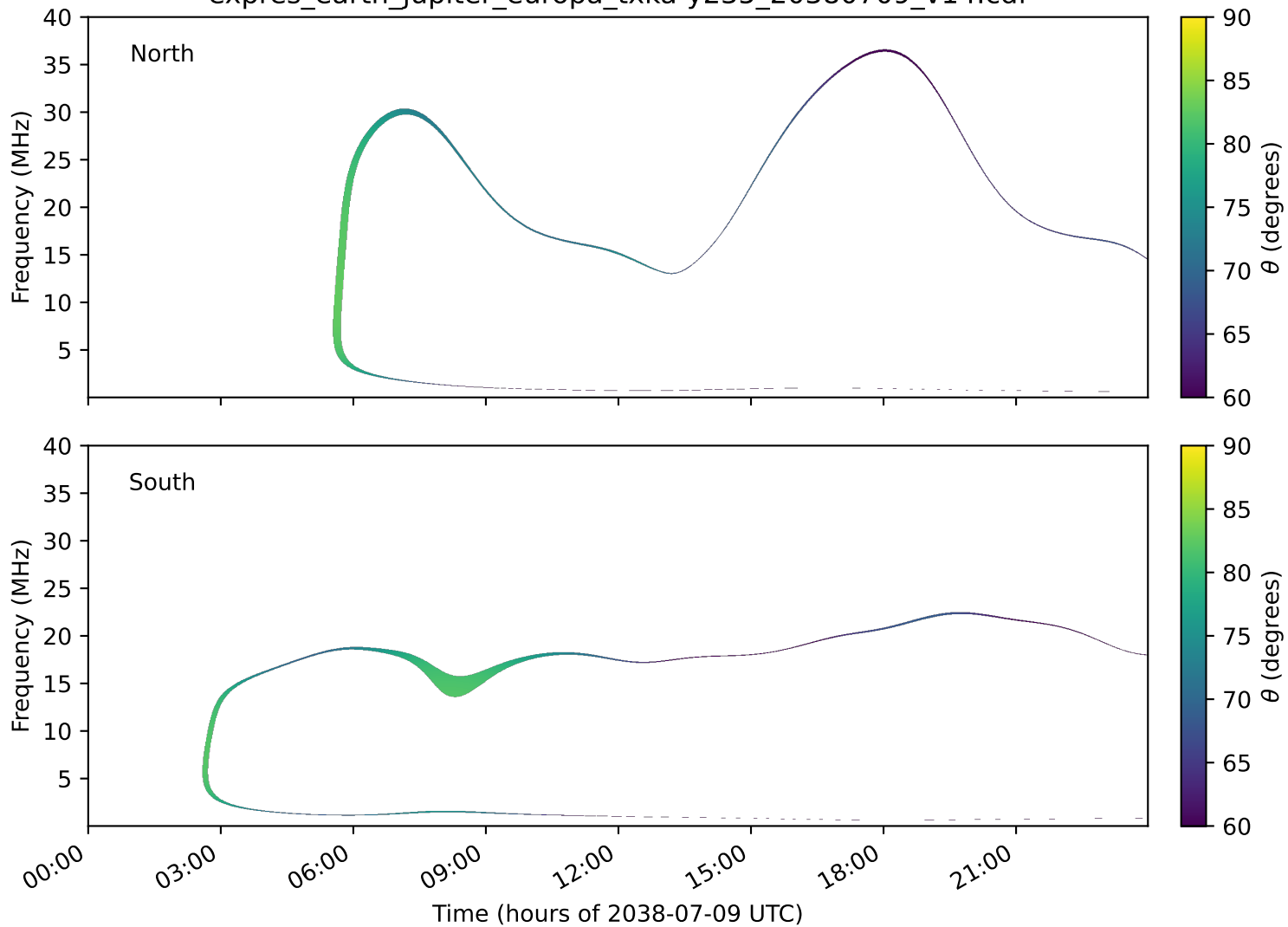
expres_earth_jupiter_europa_txka-y235_20380709_v14.cdf
