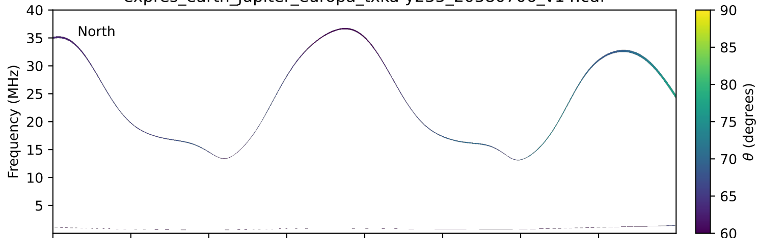
expres_earth_jupiter_europa_txka-y235_20380706_v14.cdf
