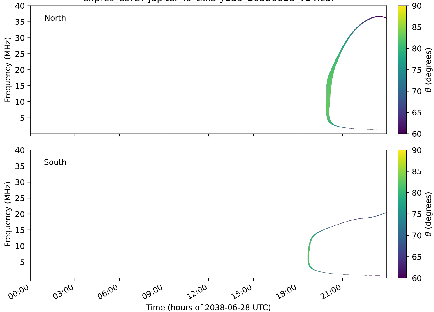
expres_earth_jupiter_io_txka-y235_20380628_v14.cdf
