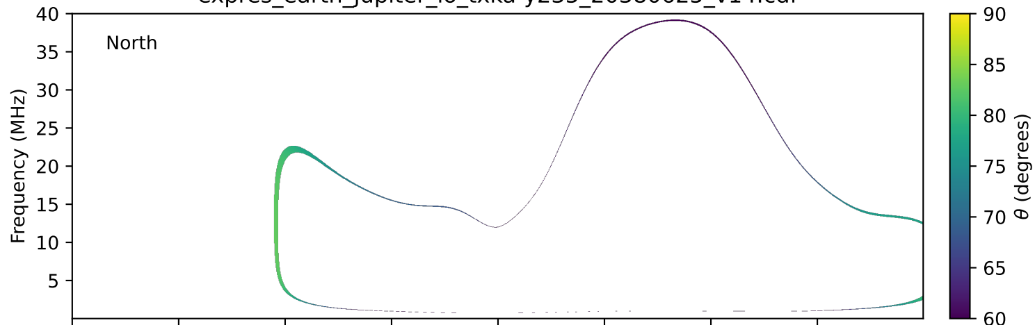
expres_earth_jupiter_io_txka-y235_20380625_v14.cdf
