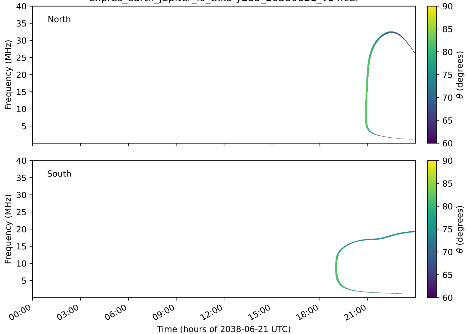
expres_earth_jupiter_io_txka-y235_20380621_v14.cdf
