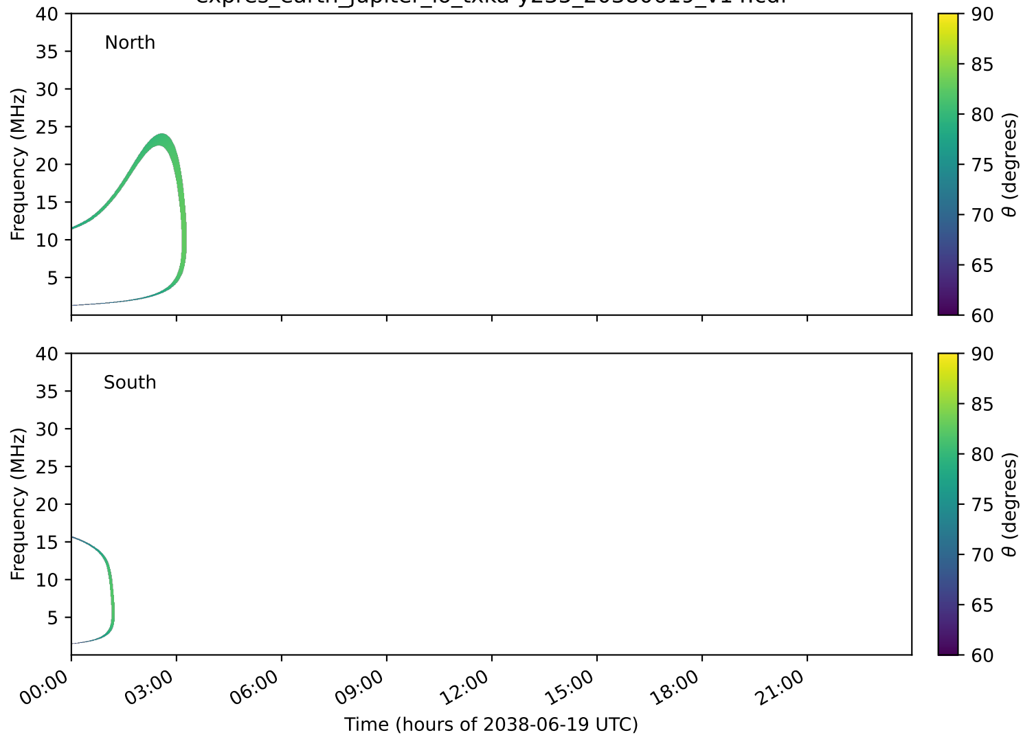
expres_earth_jupiter_io_txka-y235_20380619_v14.cdf
