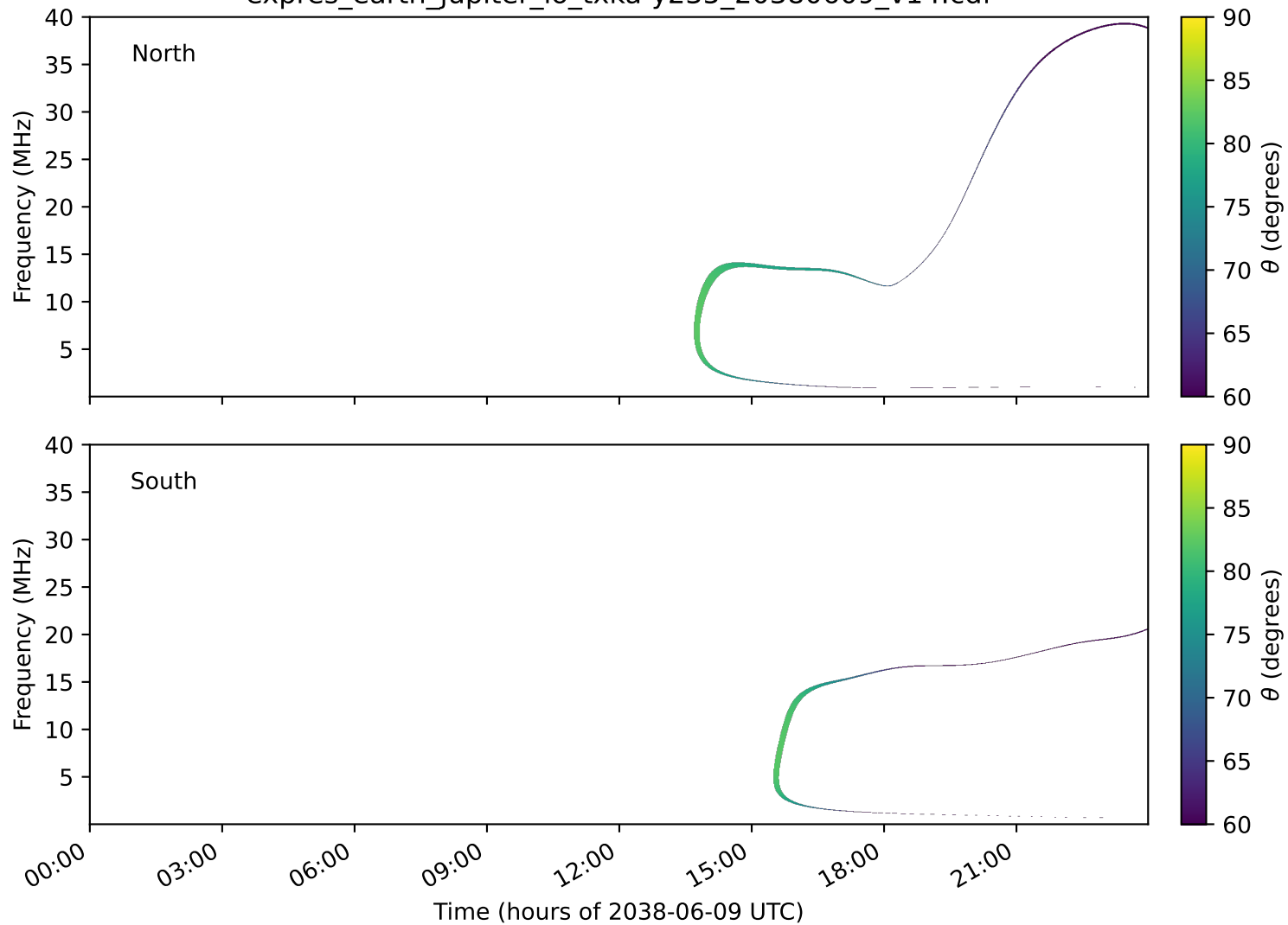
expres_earth_jupiter_io_txka-y235_20380609_v14.cdf
