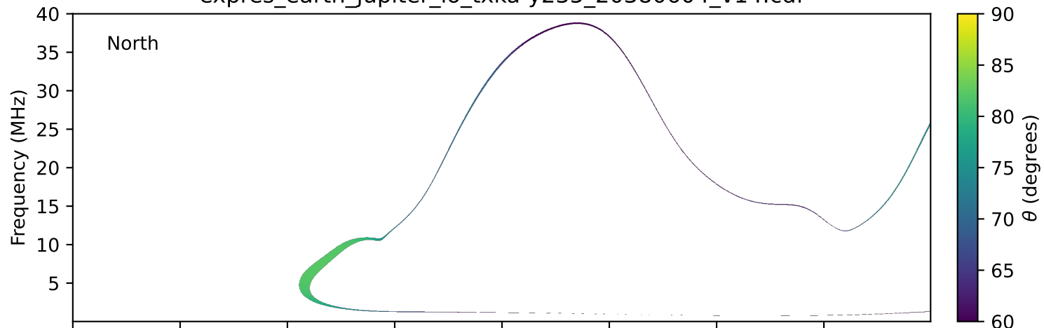
expres_earth_jupiter_io_txka-y235_20380604_v14.cdf
