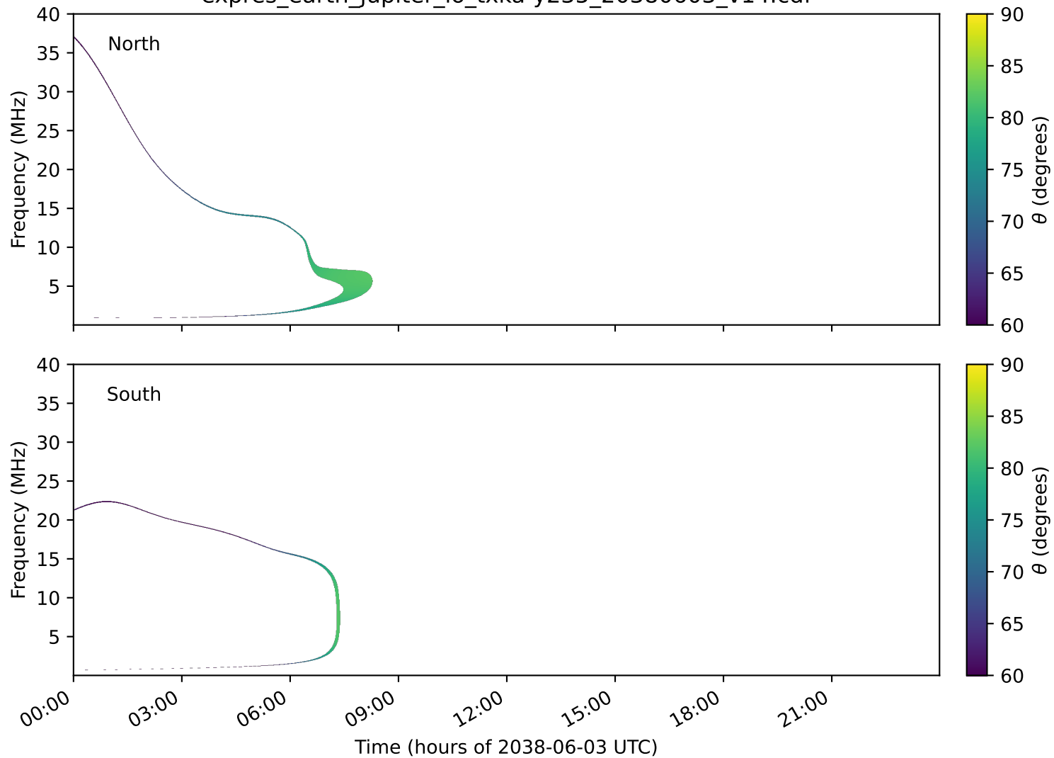
expres_earth_jupiter_io_txka-y235_20380603_v14.cdf
