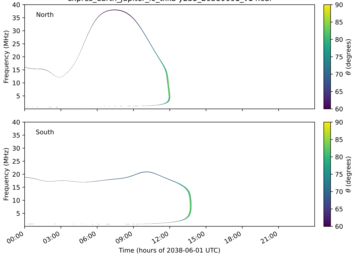
expres_earth_jupiter_io_txka-y235_20380601_v14.cdf
