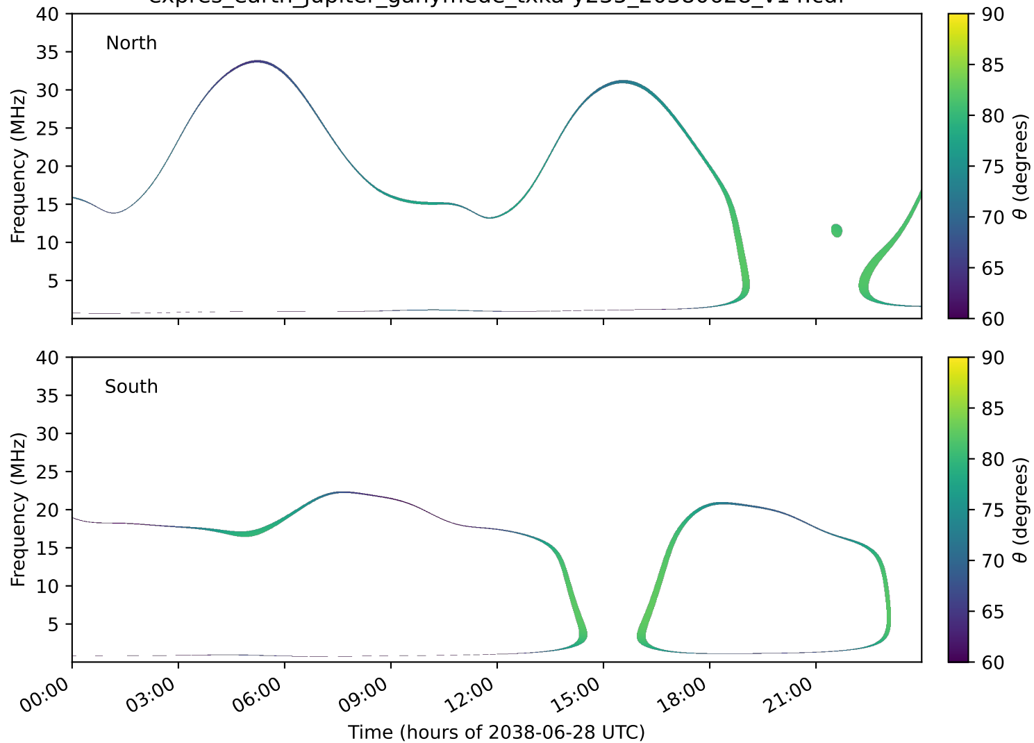
expres_earth_jupiter_ganymede_txka-y235_20380628_v14.cdf
