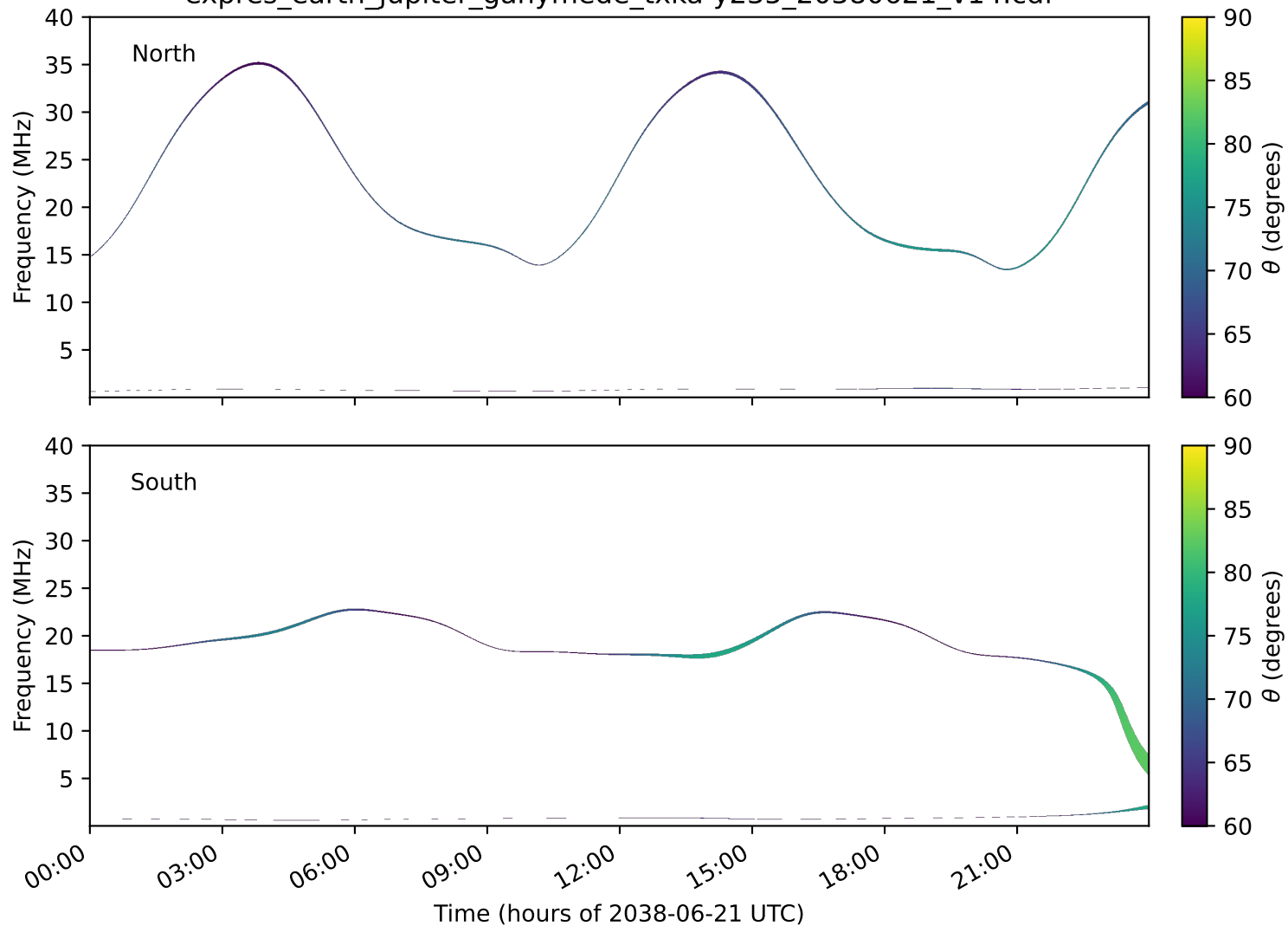
expres_earth_jupiter_ganymede_txka-y235_20380621_v14.cdf
