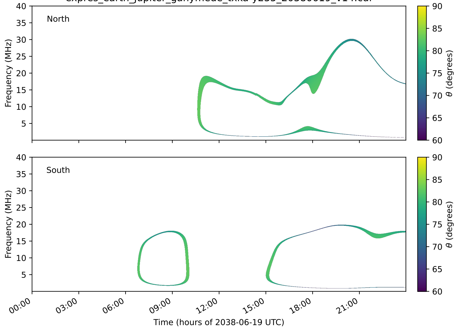
expres_earth_jupiter_ganymede_txka-y235_20380619_v14.cdf
