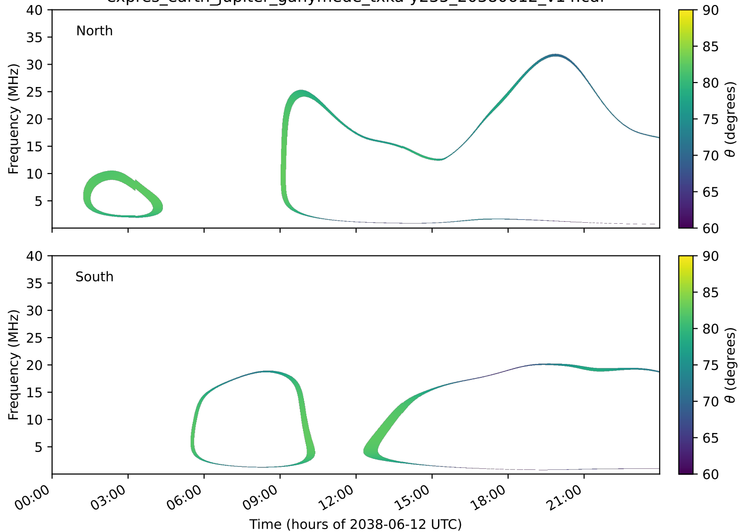
expres_earth_jupiter_ganymede_txka-y235_20380612_v14.cdf
