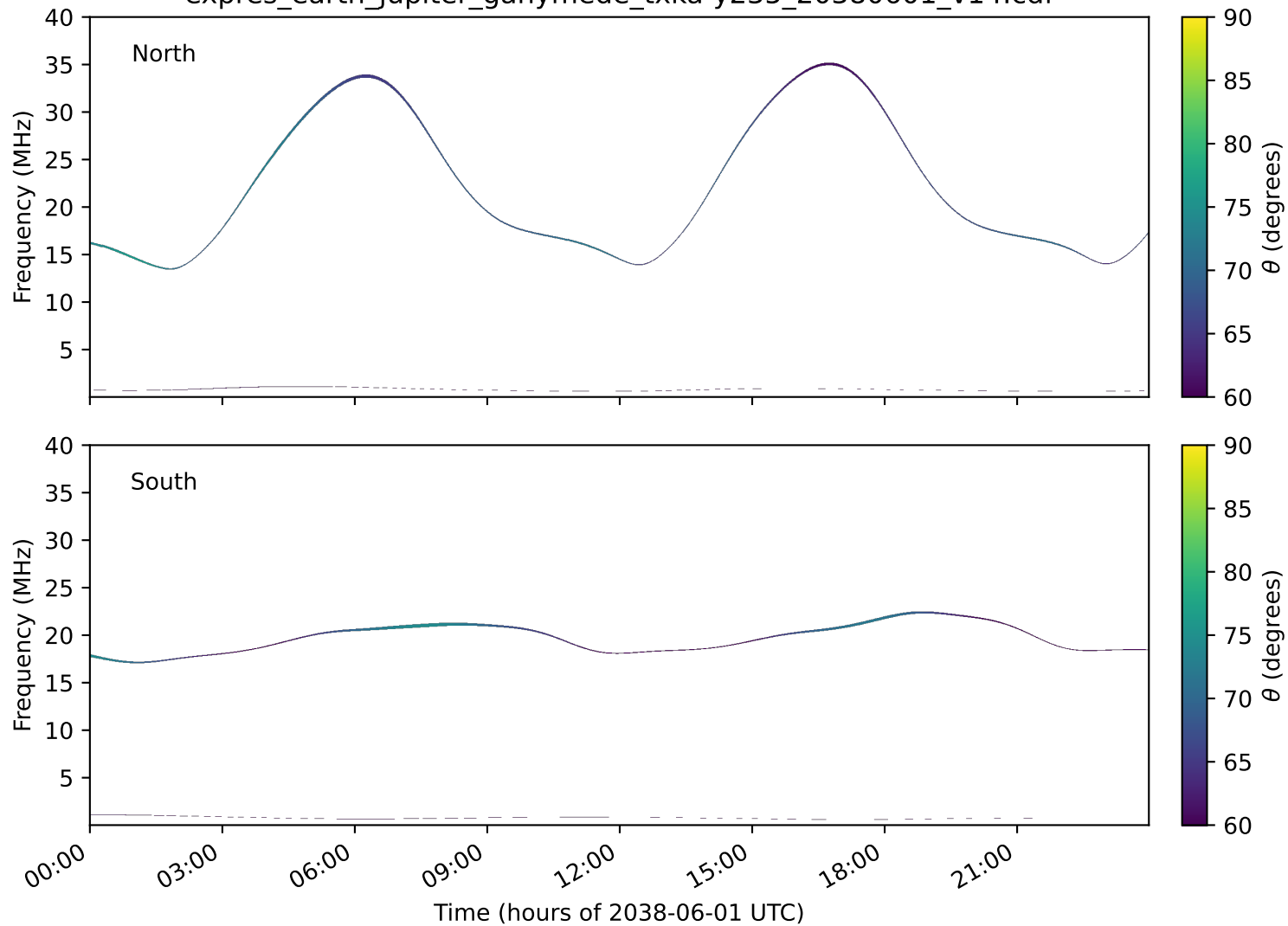
expres_earth_jupiter_ganymede_txka-y235_20380601_v14.cdf
