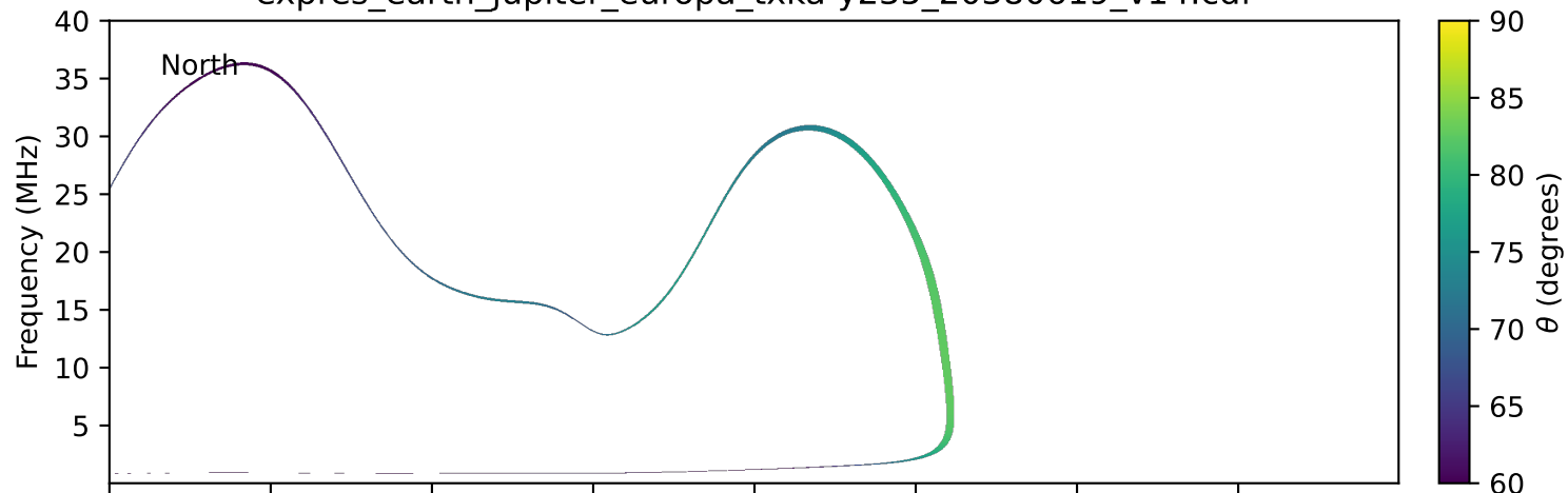
expres_earth_jupiter_europa_txka-y235_20380619_v14.cdf
